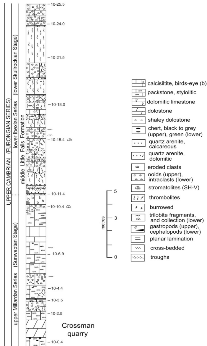
Figure 6. Cambrian stratigraphy at Stop 3 (Crossman quarry) just north of Washington County Rte 10. Conodont samples (meters above base of section) indicated by numbers to right of column (e.g., 10-10.4).
