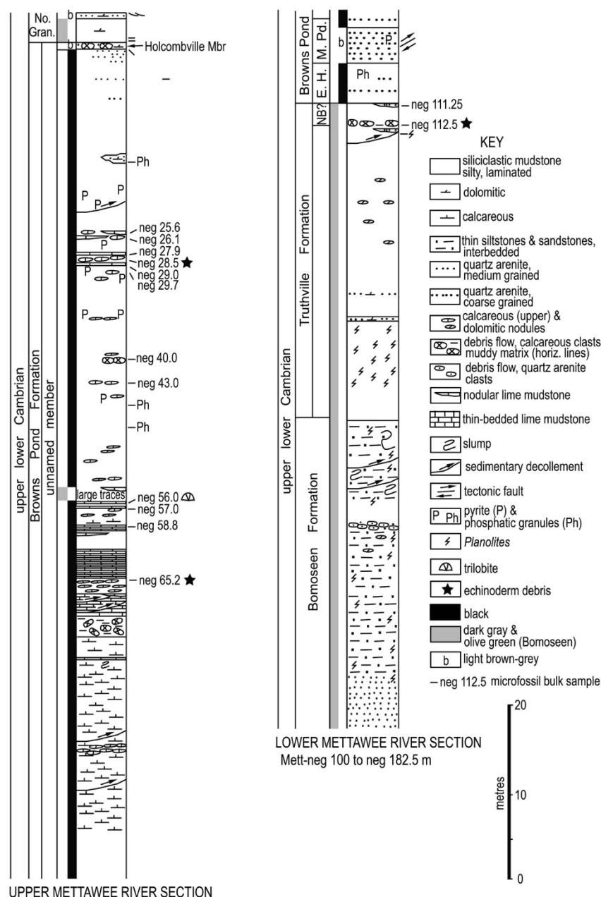
Figure 9. Section along the Mettawee River downstream from the falls on the Bomoseen Formation to c. 0.6 km upstream from the Lower Turnpike bridge at North Granville village, N.Y. Abbreviations: E.H., Eddy Hill Member; M. Pd., Mudd Pond Member; No. Gran., North Granville Formation.
